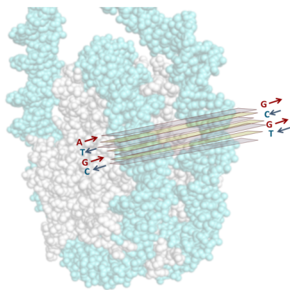
Two DNA loops in nucleosome
