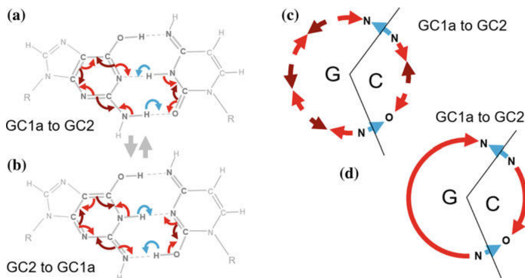
Fig. 5 Tautomeric transition GC1a to GC2. Proton relocations are in blue. Relocations of individual electrons in the same direction as protons are in brown and relocations in the opposite direction are in red. a Transition GC1a to GC2. b Transition GC2 to GC1a. c Simplified summary of charge relocations GC1a to GC2. d Even more simplified summary of charge relocations GC1a to GC2
