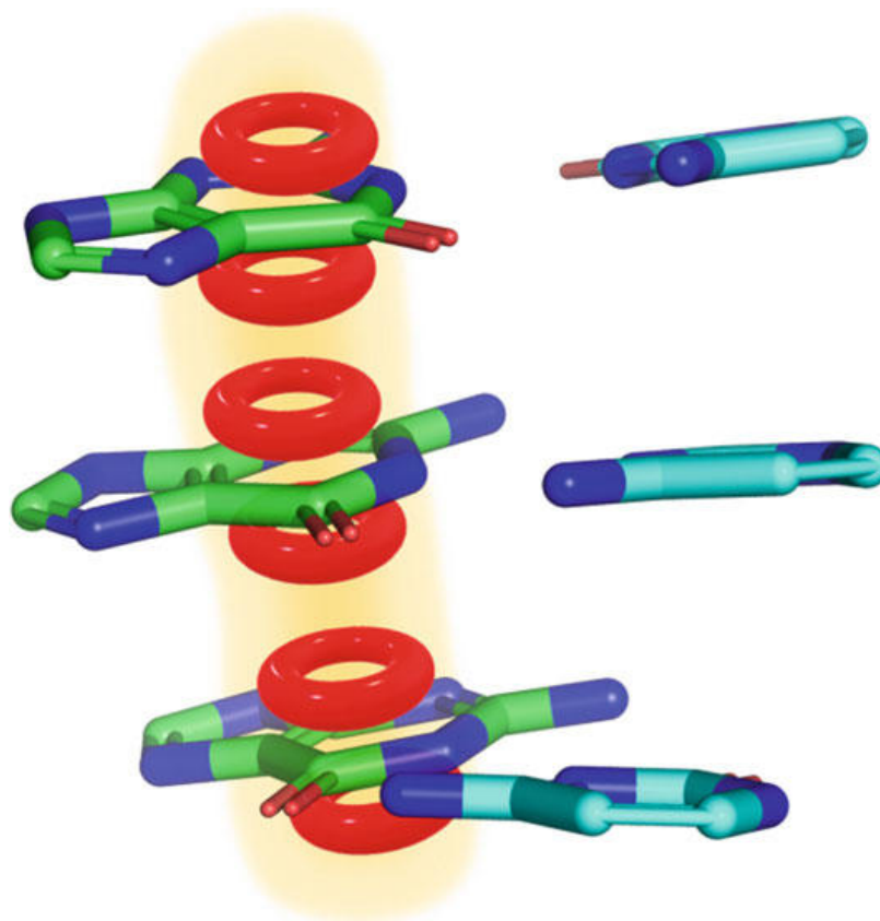
Fig. 3 Aromatic electron rings are merged in a purine stretch. Three basepairs of the basestack are shown. The backbone is hidden. Aromatic pi electrons of the central rings are shown in red. A cloud of delocalized aromatic electrons is shown in yellow
