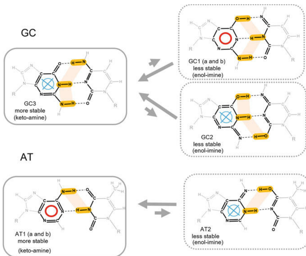
Fig. 8 Stability and aromaticity oscillations of purine tautomers in basepairs
