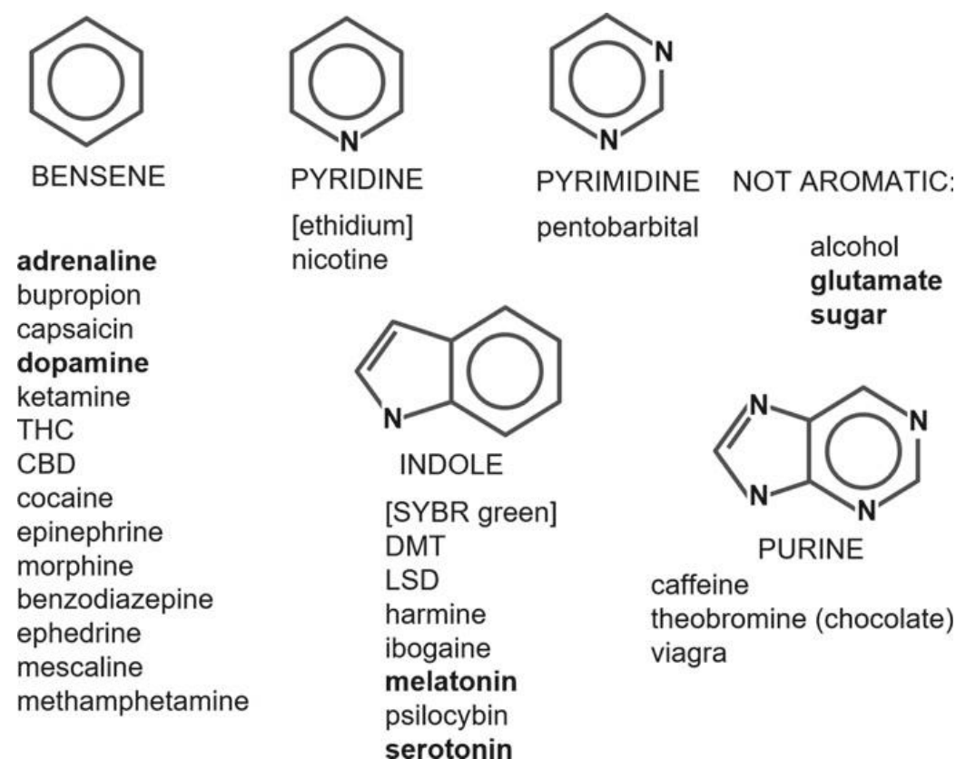
Fig. 7 Aromatic groups and exogenous and endogenous psychoactive substances classified by the aromatic groups they contain. In bold are endogenous psychoactive substances. In square brackets are intercalating substances widely used in DNA research, for which psychoactive properties are unknown. Only the benzene, pyridine, pyrimidine, indole, and purine groups are shown. All the psychoactive substances listed underneath contain additional, sometimes also aromatic, radicals which are not shown
