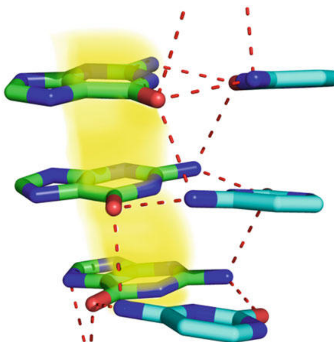
Fig. 6 Electron clouds and proton wires in DNA. A stretch of purines in the double helix is shown. It is a GGG sequence, GGG is shown in green and the complementary strand CCC in aqua color. The DNA backbone is not shown. The electron cloud is shown in yellow. Proton wires are shown in dotted lines
