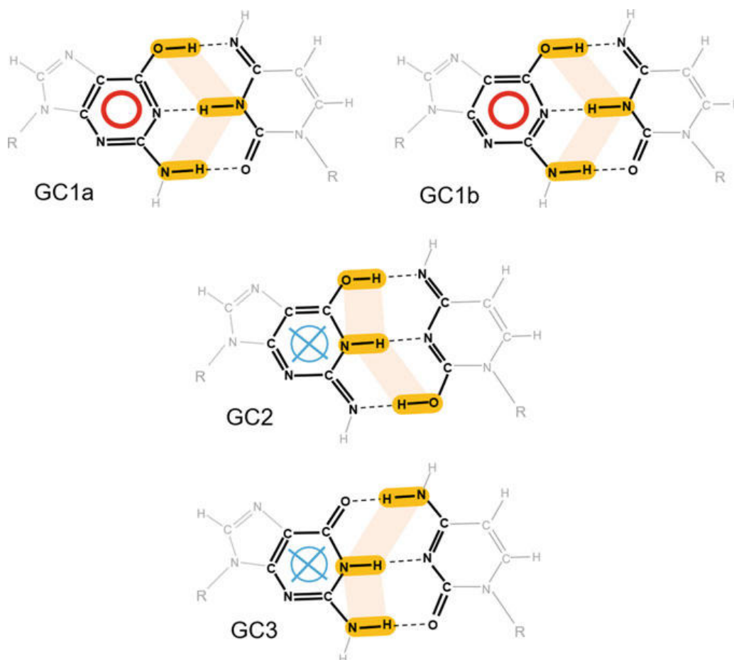
Fig. 1 Tautomeric forms of GC basepair. The hexagonal heterocycles of purines are called here “the central ring” and labeled with circles. The uncrossed circles signify the presence of aromaticity and the crossed circles signify the loss of aromaticity. The remaining heterocycles are not aromatic. The black lines signify the structures that undergo tautomerization and grey lines signify the structures that stay unchanged during tautomerization. Links to the backbone are shown as “R”
