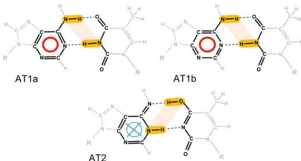
Fig. 2 Tautomeric forms of basepair AT
